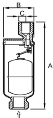
No.11AV DIMENSIONS (MM). MOP(KG/CM 2 ). WT(KG)
